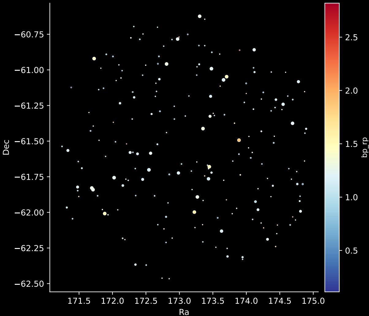
APOGEE DR17 Field: [272-38-O_TESS] Stars: 201
