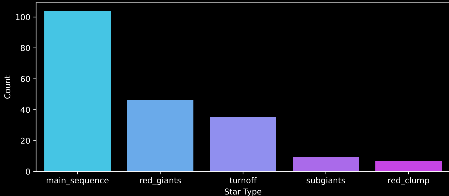
APOGEE DR17 Field: [272-38-O_TESS] Count plot of Star Type
