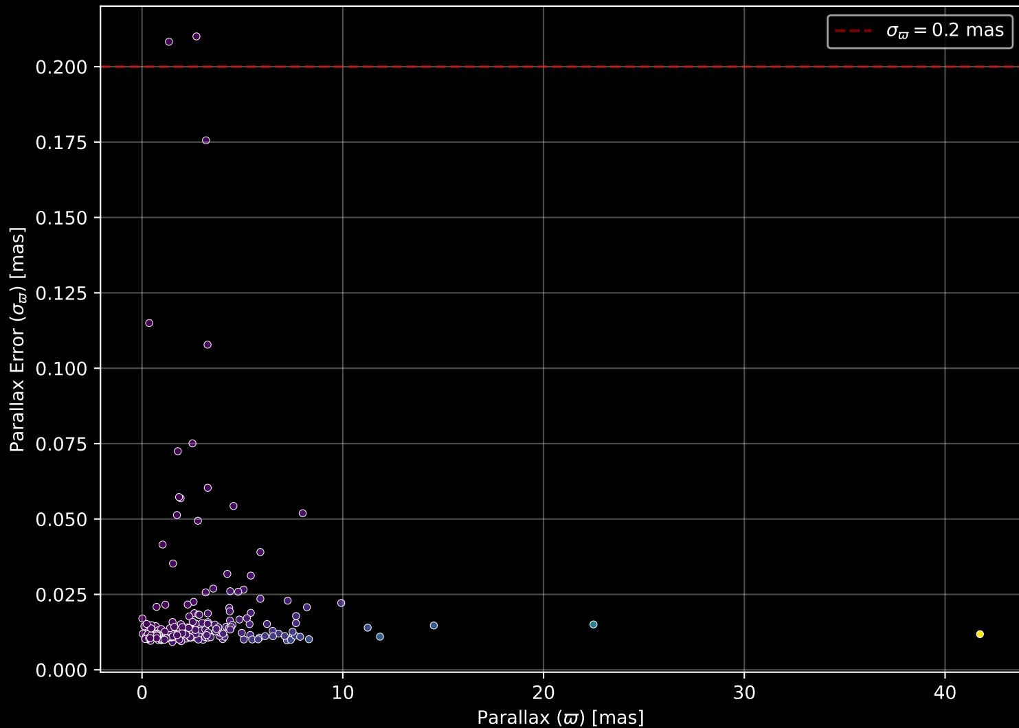
APOGEE DR17 Field: [272-38-O_TESS] Parallax Quality (n= 201)
