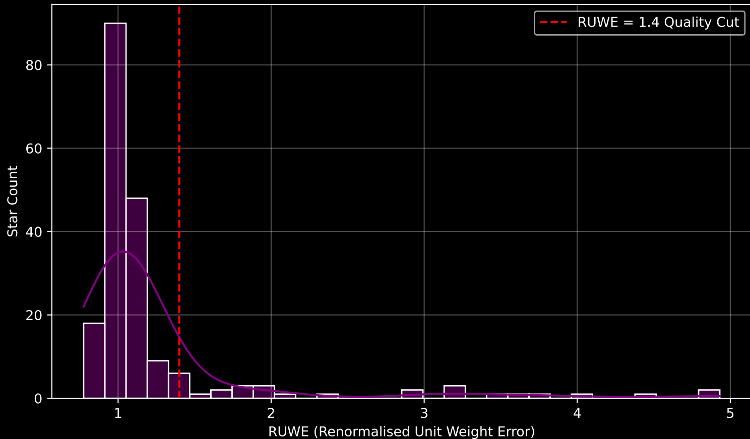
GAPOGEE DR17 Field [272-38-O_TESS] RUWE Distribution (n= 194)
