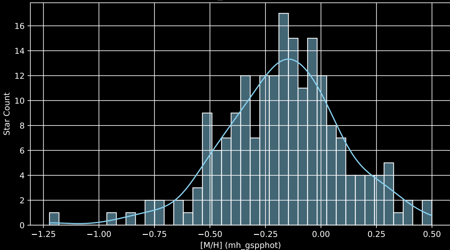
APOGEE DR17 Field: [272-38-O_TESS [M/H] (mh_gspphot) (n= 198)
