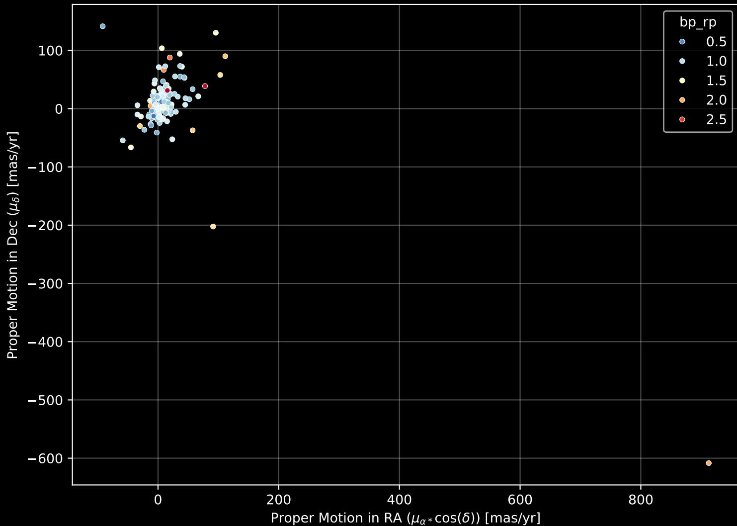
APOGEE DR17 Field: [272-38-O_TESS] Proper Motion Diagram (n= 201)
